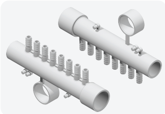
Part #: 72082 (8) 3/8" barbs x 1" SPG x 1"S with cap
