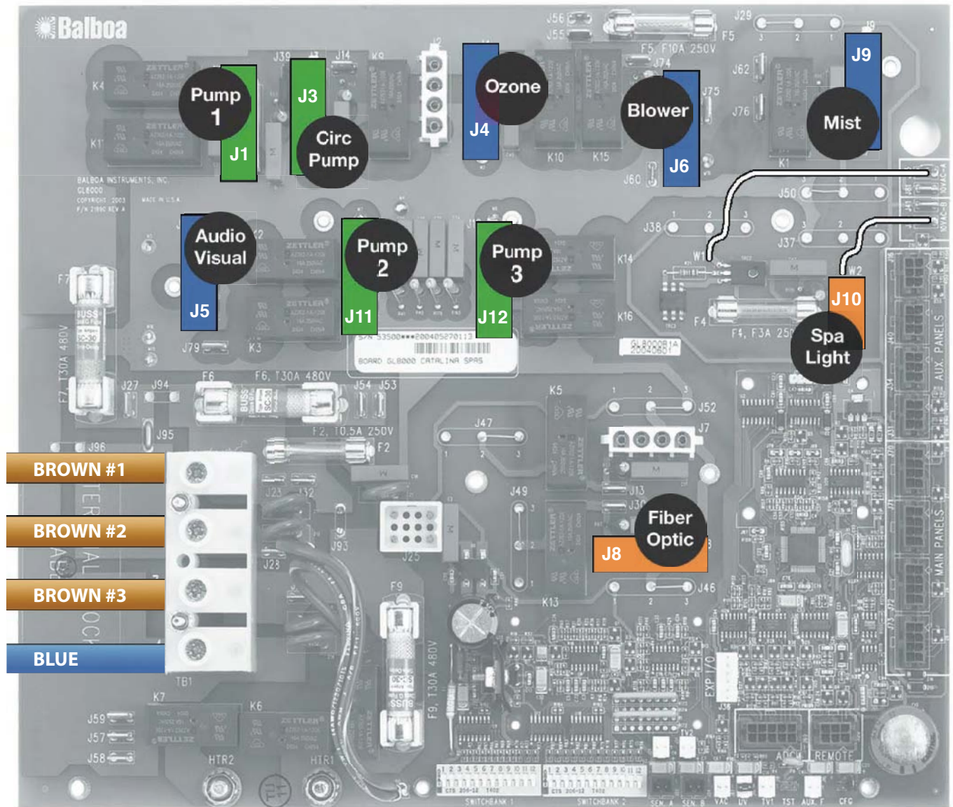
Three Service Connection Shown Above (3 Lines + 1 Neutral)
